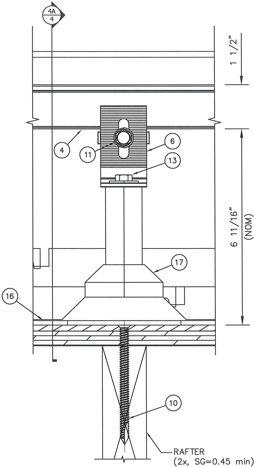
2 2 QB-1 DETAIL
